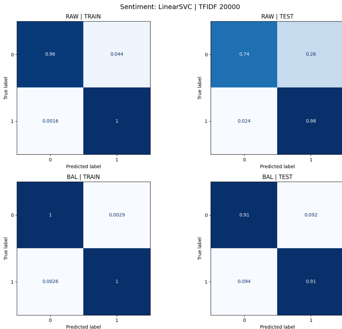
Slika 9: Matrice konfuzije – LinearSVC, TF-IDF 20k, cilj Sentiment (RAW i BAL, train i test)
